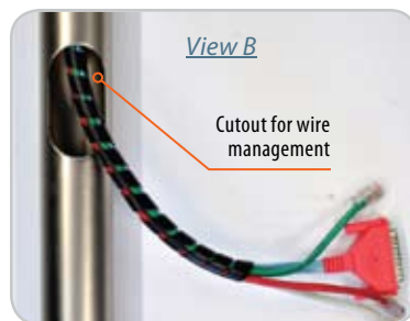
View B Steel pole with cutouts (two front and one rear) for wire management
