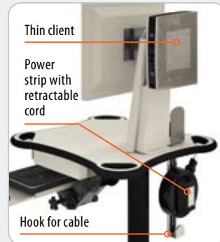
Supports separate thin client and monitor
