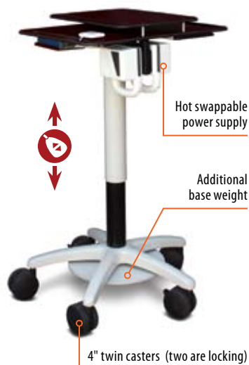
Laptop Cart # LPC200 with laptop lock shelf
