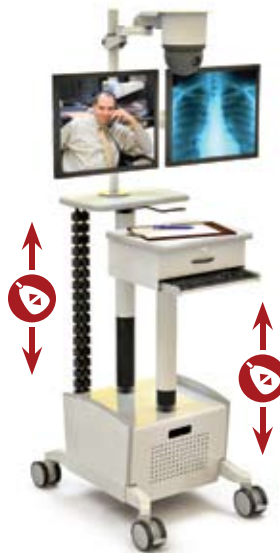
D. Telemedicine Cart XPC1926 with two pneumatically height-adjustable drives and camera shelf on Z-arm
