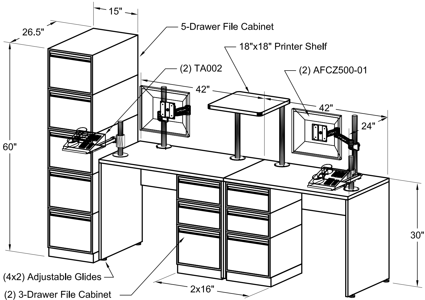
ISOMETRIC VIEW
