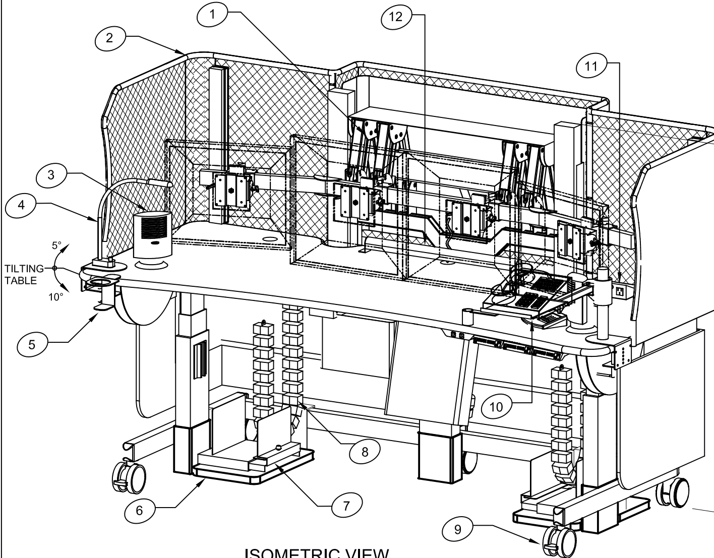
ISOMETRIC VIEW
