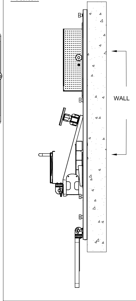
SIDE VIEW OF UNIT IN FOLDED POSITION
