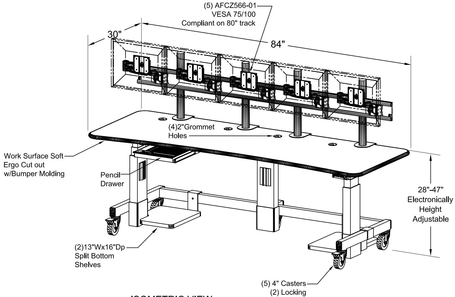
ISOMETRIC VIEW
