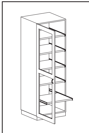
FC 24"W x 24"D x 72"H
