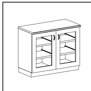
FC 36"W x 18"D x 30"H
