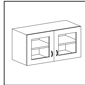
WC 36"W x 16"D x 18"H
