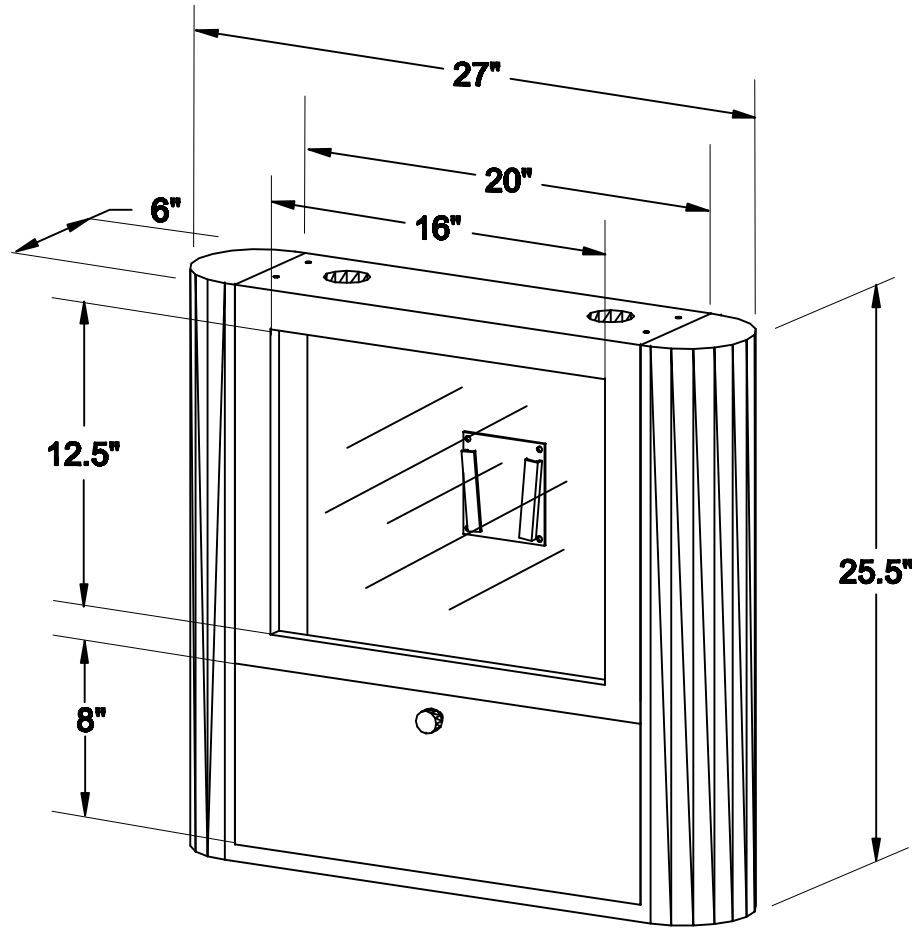
ISOMETRIC VIEW
